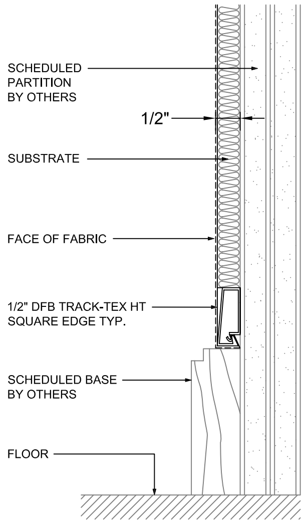
Base Detail - Wood
