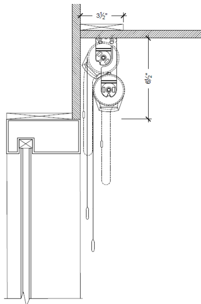
Ceiling or Wall Mount Double No Attachments
