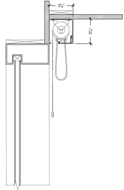
Ceiling or Wall Mount Single with Pocket
