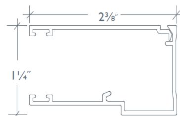
Side Channel for Blackout
