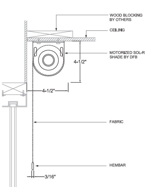
Ceiling or Wall Mount Single No Attachments
