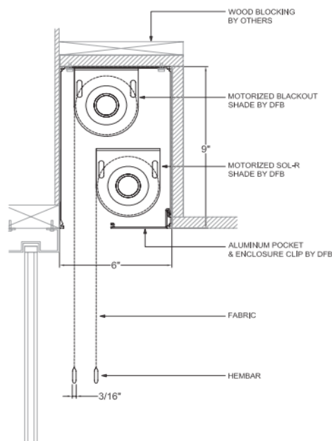
Piggyback Ceiling or Wall Mount Recessed with optional Pocket
