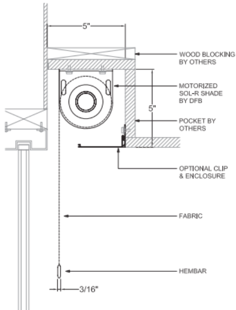
Ceiling or Wall Mount Single Recessed with Clip & Enclosure
