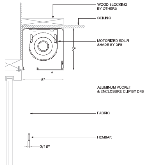
Ceiling or Wall Mount Single with Pocket
