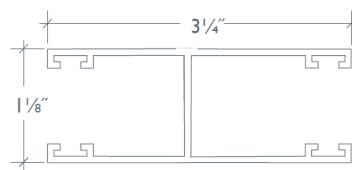
Center Channel for Blackout
