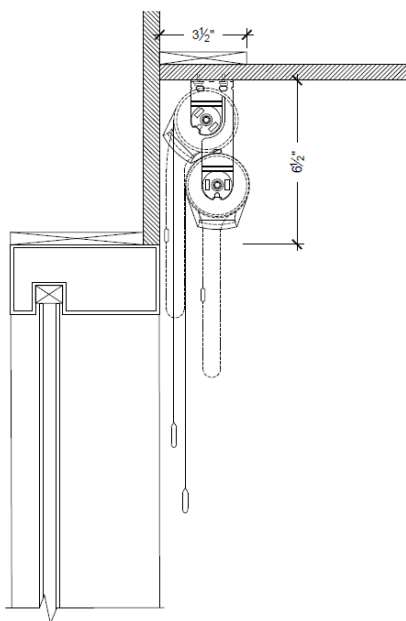
Ceiling or Wall Mount Double No Attachments
