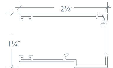
Side Channel
