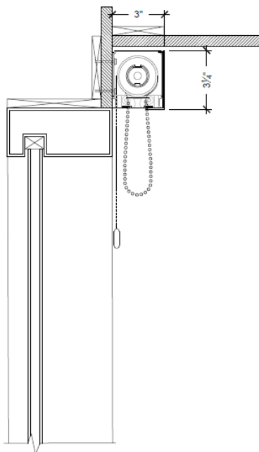
Ceiling or Wall Mount Single with Facia
