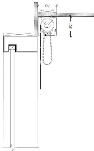
Ceiling or Wall Mount Single with Pocket
