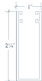
Sill Channel
