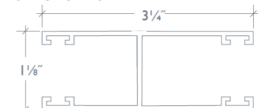
Center Channel
