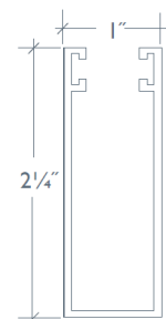
Sill Channel
