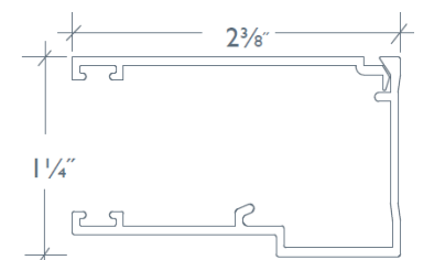
Side Channel
