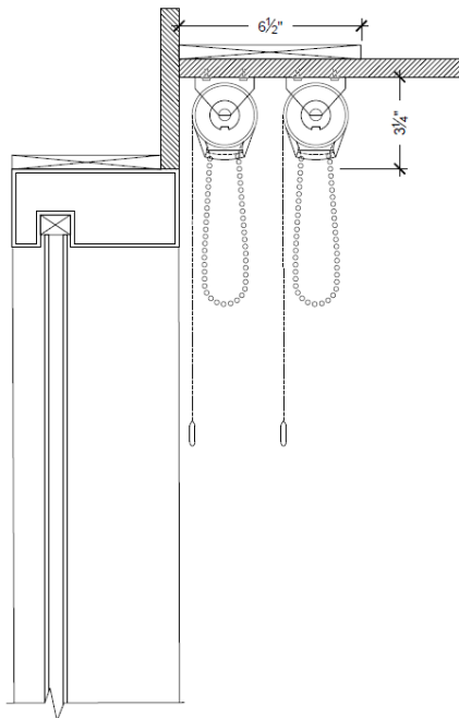
Side by Side Ceiling or Wall Mount Double. No Attachments
