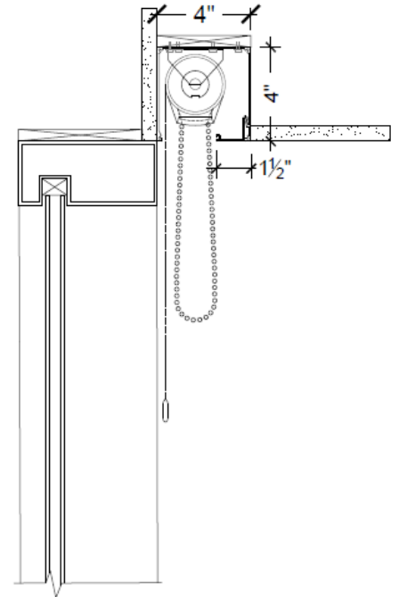
Ceiling or Wall Mount Single with Aluminum Pocket
