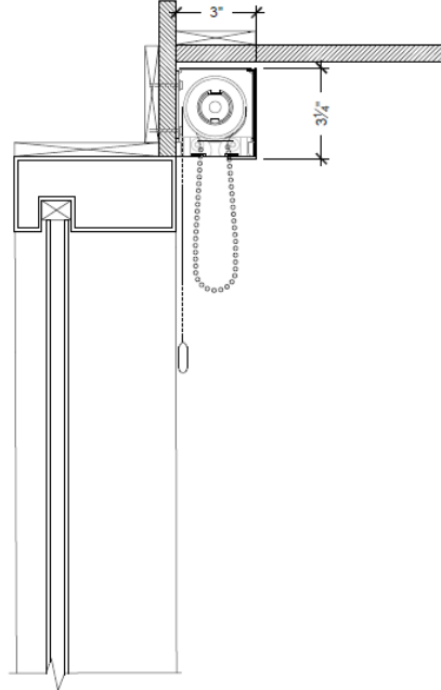
Ceiling or Wall Mount Single with Fascia
