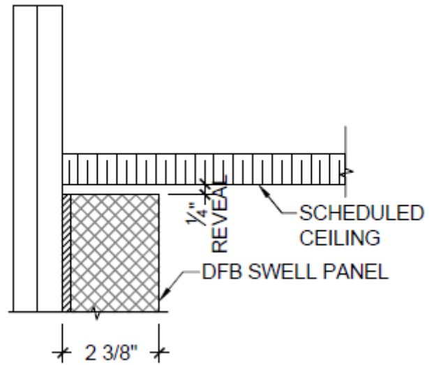
SWELL Acoustical Panel™ CEILING SECTION DETAIL
