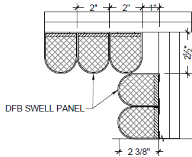
SWELL Acoustical Panel™ CORNER CONDITION DETAIL
