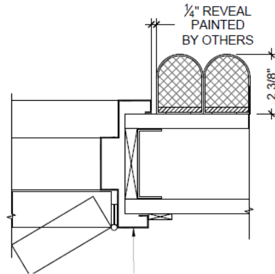
SWELL Acoustical Panel™ DOOR CONDITION DETAIL
