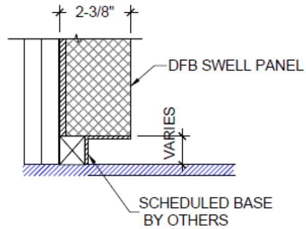
SWELL Acoustical Panel™ FLOOR SECTION DETAIL
